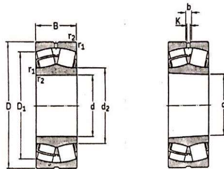
Cylindrical bore
